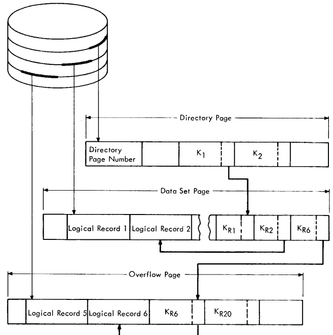
Figure 23. Typical Virtual Index Sequential Data Set
