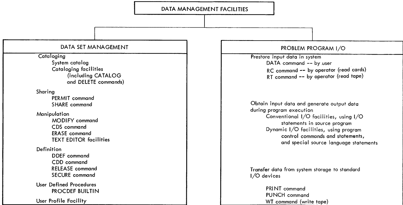
Figure 20. Time Sharing System/360 Data Management Facilities
